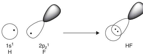
Figure 1.16 VB model of HF
