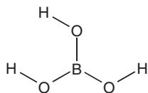
Figure 4.3 Chemical structure of boric acid
