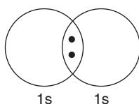
Figure 1.15 VB model of H_2
