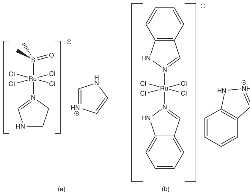
Figure 7.50 Chemical structures of and (a) NAMI-A and (b) KP1019
