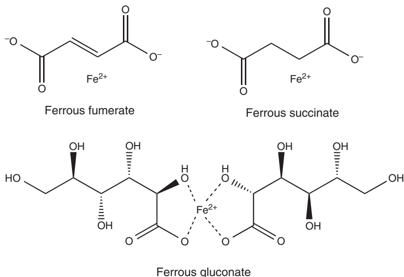
Figure 7.47 Chemical structure of Fe(II) fumarate, Fe(II) succinate and Fe(II) gluconate
