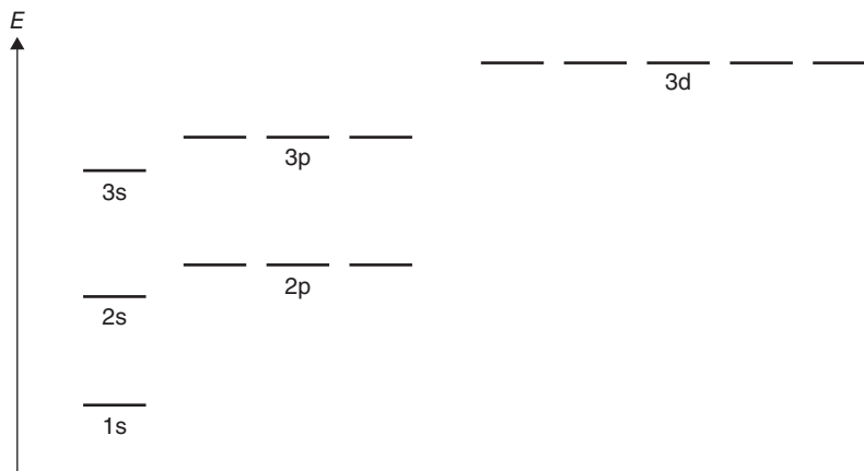
Figure 1.9 Energy diagram
