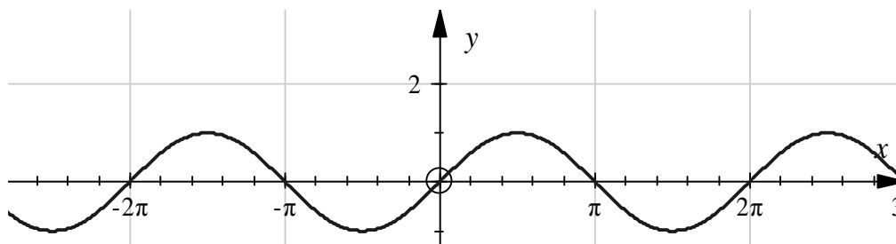
Figure 9.2 Graph of y = \sin x
