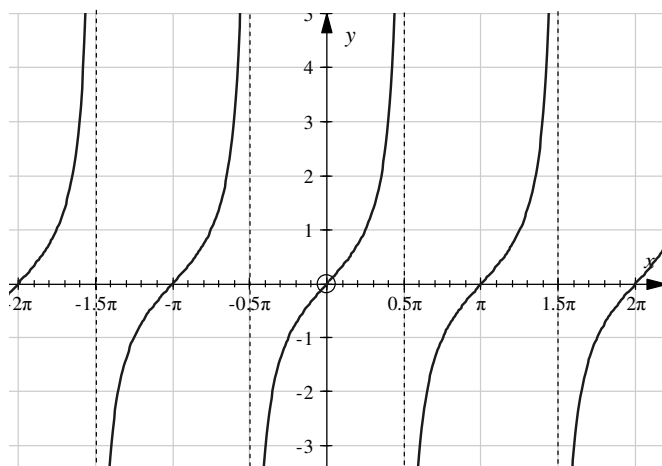
Figure 9.3 Graph of y = \tan x
