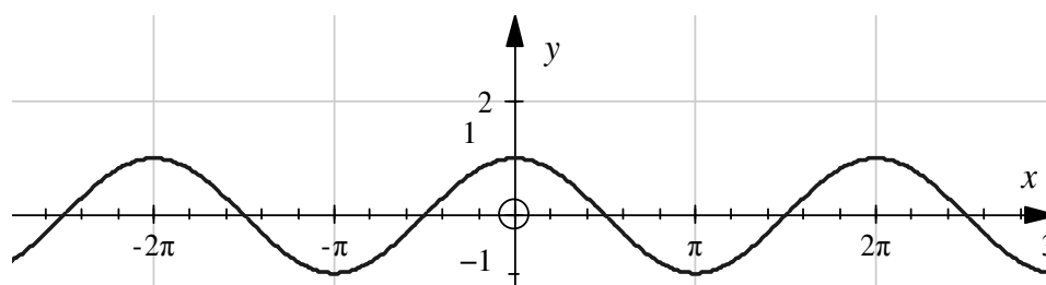
Figure 9.1 Graph of y = \cos x
