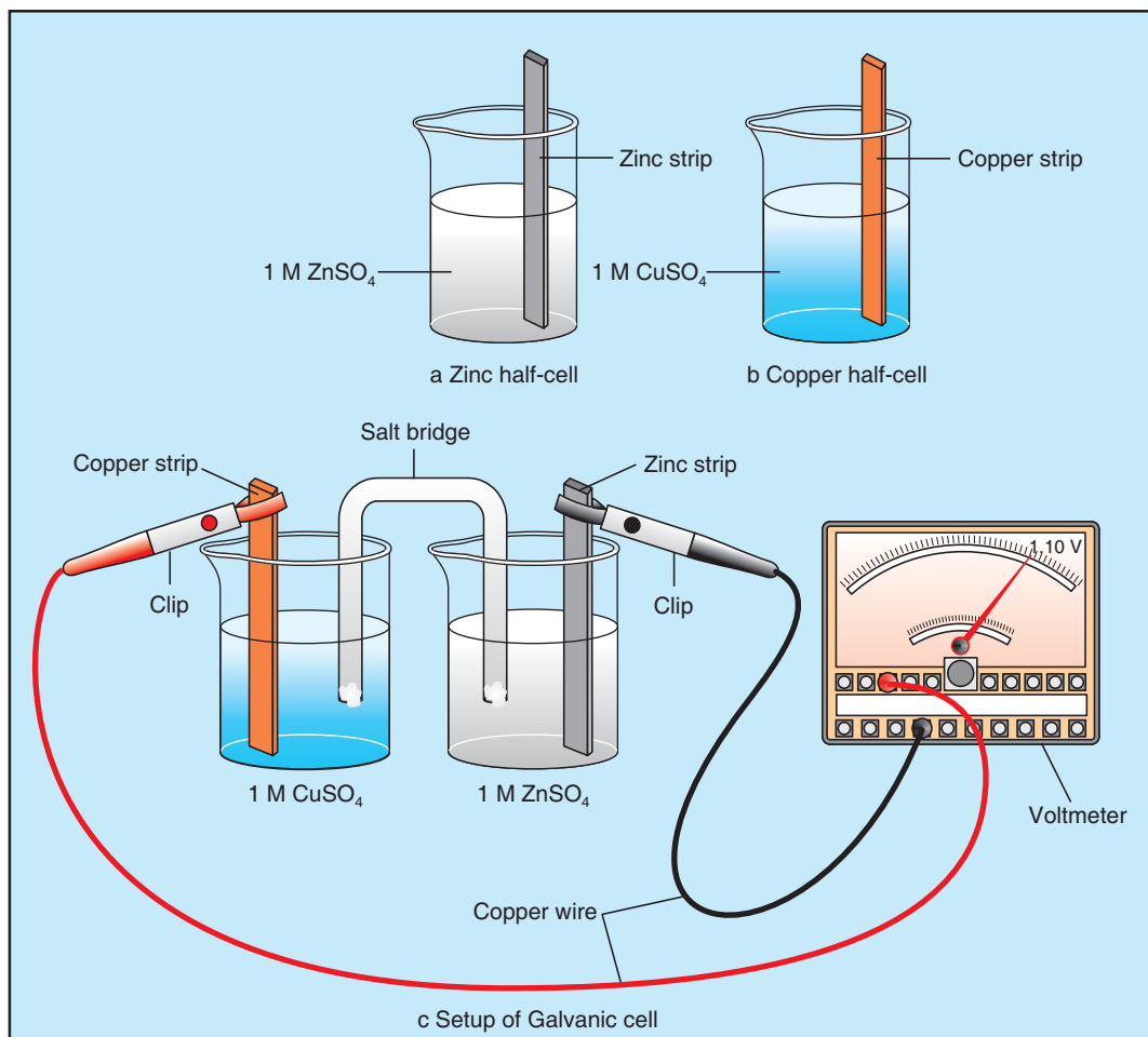
Figure 4.9 Daniell Cell.
