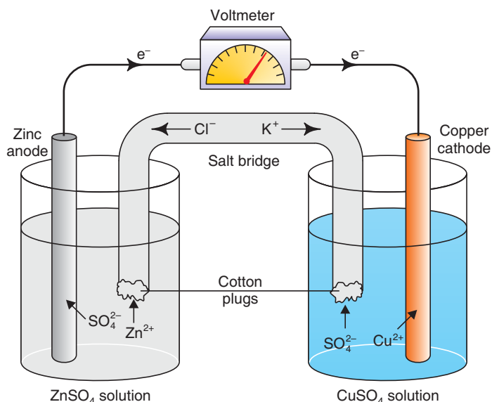
Figure 4.7 Daniell cell.
