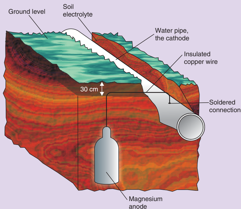
Figure 4.14 Protection of iron using magnesium.
