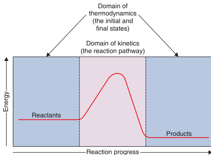
Figure 3.1 Concerns of kinetics and thermodynamics.
