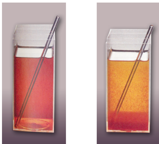
Figure 1.1 a) Solution b) Suspension
