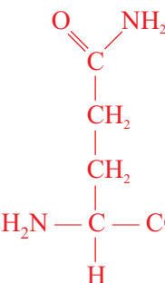
Glutamine (Gln, Q)
