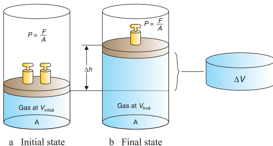
Figure 3.3 a The piston, moving a distance \Delta h against a pressure P , does work on the surroundings.
