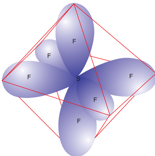
Figure 3.21 The sp^3d^2 hybrid orbitals \text{SF}_6 .
