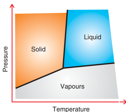
Fig. 5.8 Sketch of phase diagram of one component system.
