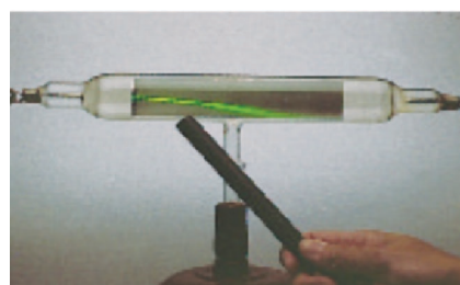
(b) The cathode ray is bent in the presence of a magnet.
