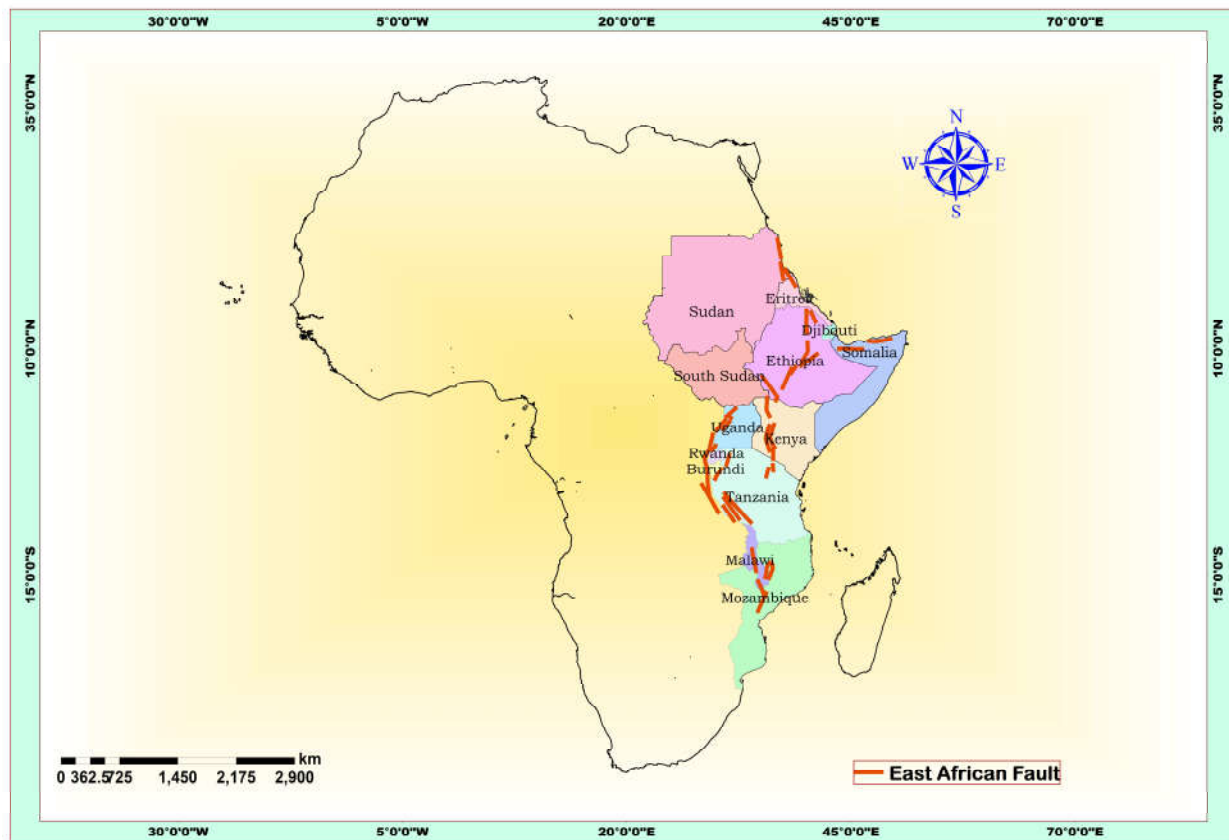
Figure 2.2. The Ethiopian and East African Rift Valley systems
