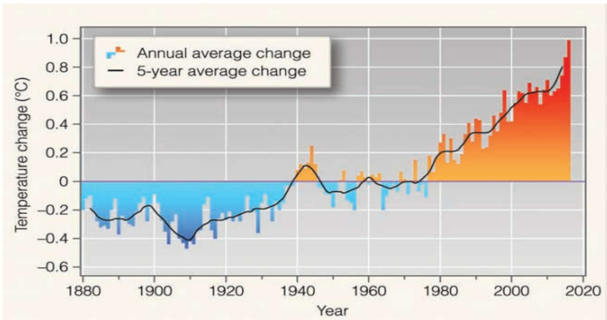
Figure 5.2: Global mean temperature anomaly.
