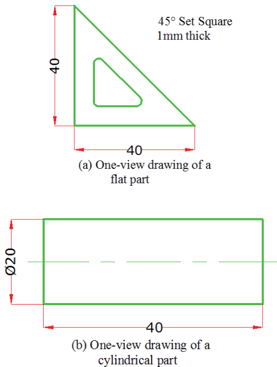
Fig. 6.16 Example of one-view drawings
