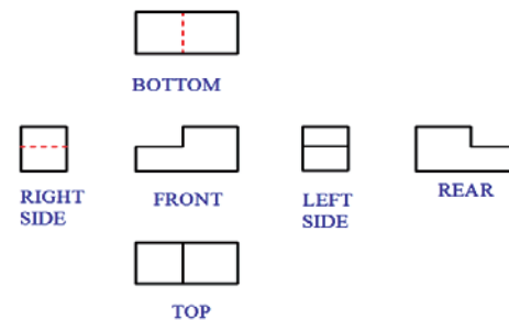
Fig. 6.11 The six principal views and their arrangement in first angle projection
