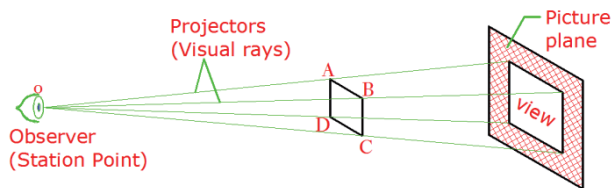
Fig. 7.1 Principle of central projection
