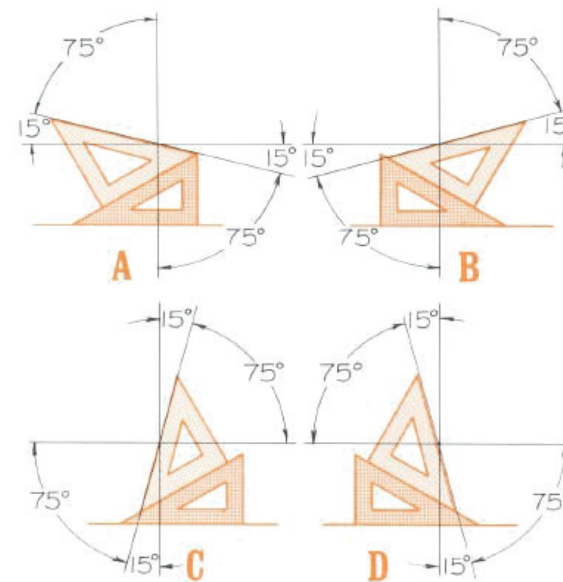
Fig. 2.27. Inclined lines using 45^\circ & 30-60^\circ set squares
