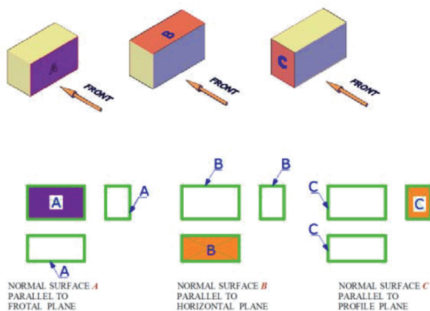
Fig. 6.24 Normal surfaces
