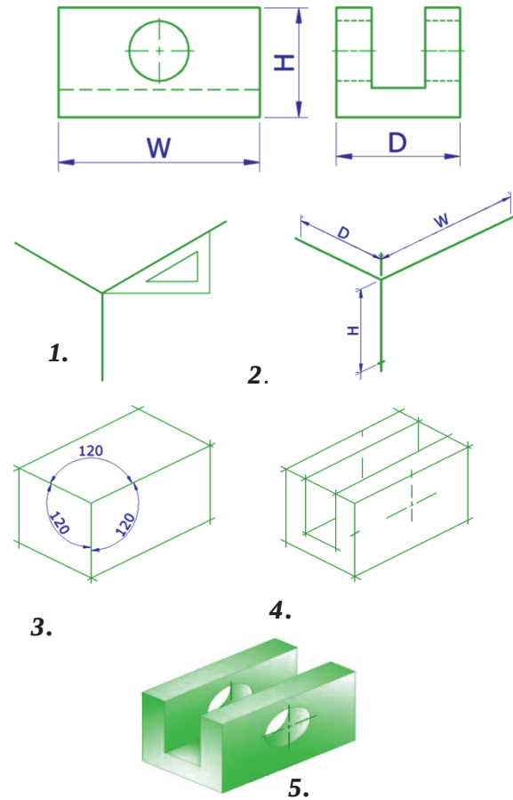
Fig. 7.23 Construction of isometric drawing
