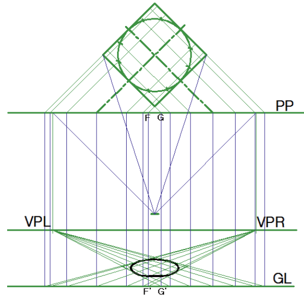
Fig. 7.47 Construction of circle on horizontal plane
