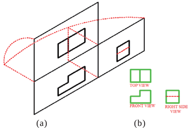
Fig. 6.8 Projection planes unfolded
