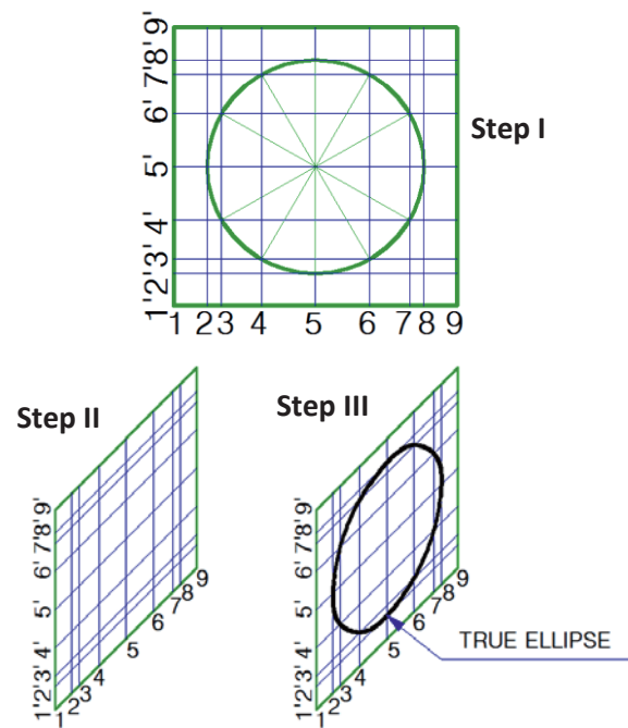
b) Grid construction method
