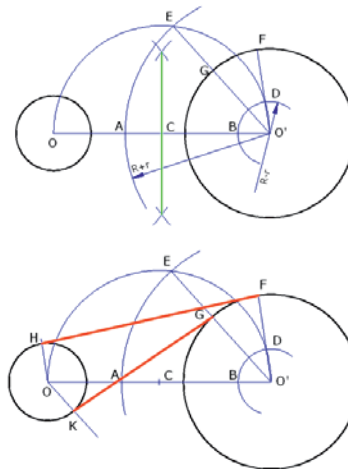
Fig. 5.37 Constructing tangent line to two circles of different size
