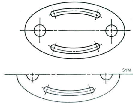
Fig. 3.4 Center lines
