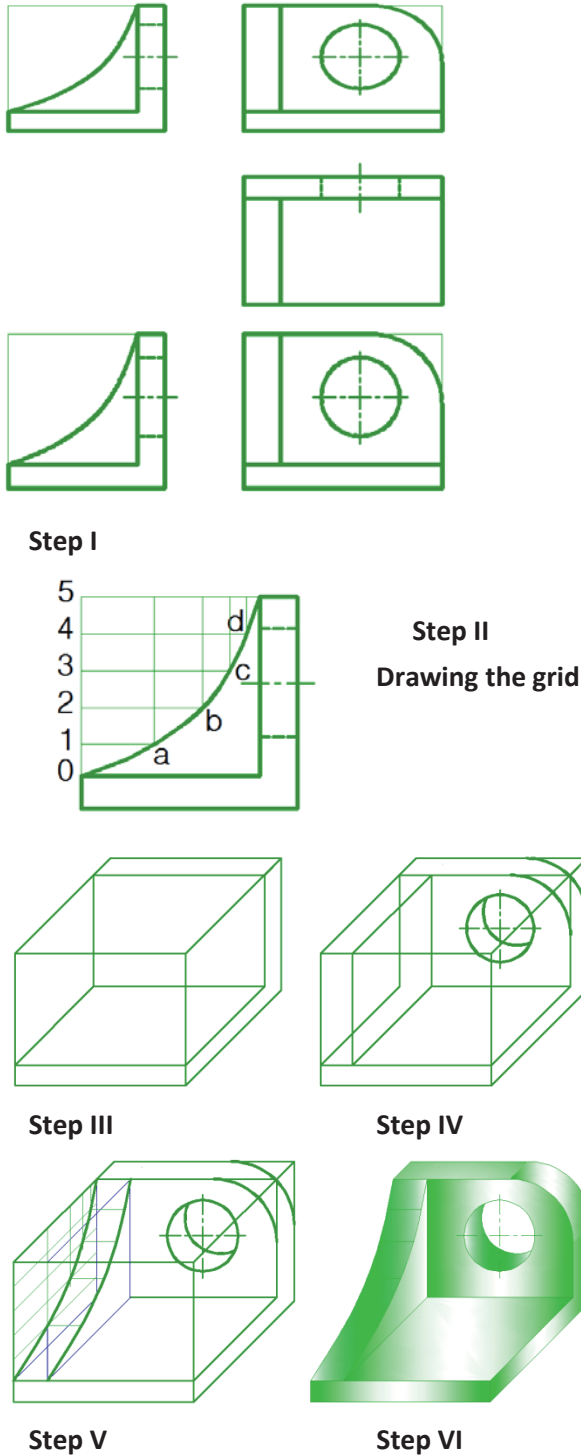
Fig. 7.30 Construction of oblique drawing using box method
