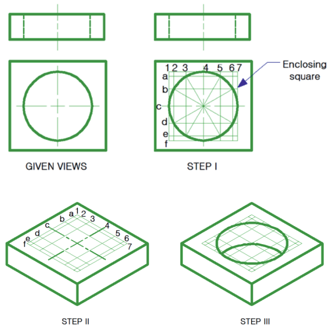
Fig. 7.17 Construction of isometric circles by offset measurement
