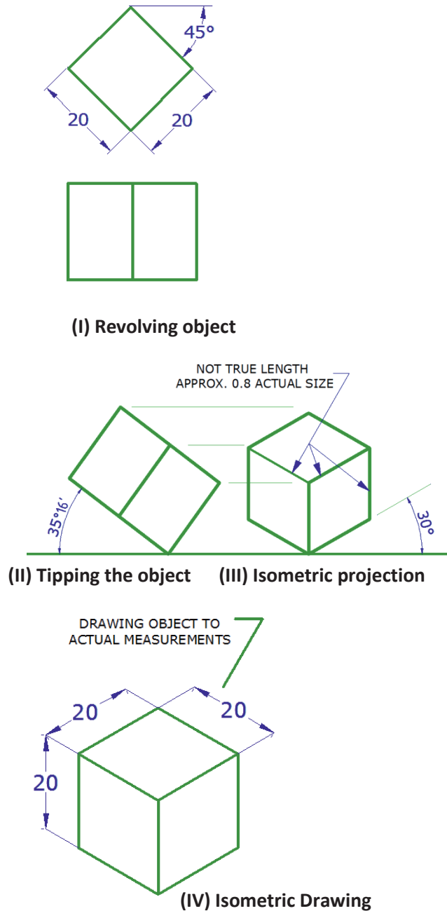
Fig. 7.8 Isometric projection
