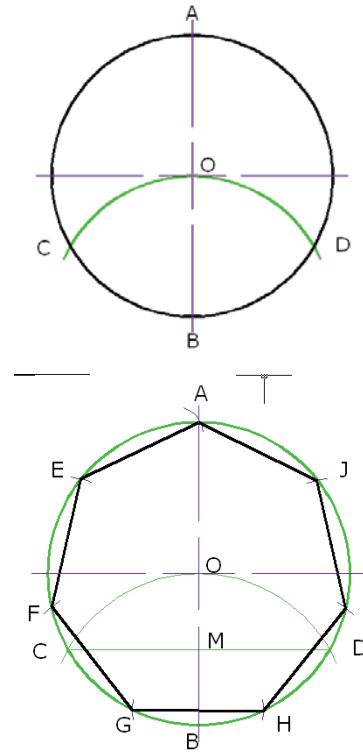
Fig. 5.31 Constructing a regular heptagon given the circumscribing circle
