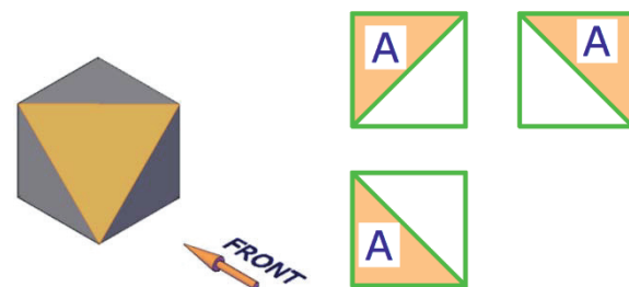
Fig. 6.27 Projection of oblique surface
