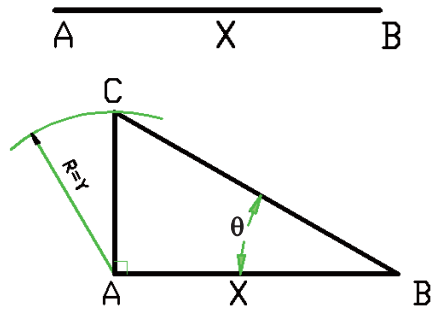
Fig. 5.12 Tangent method
