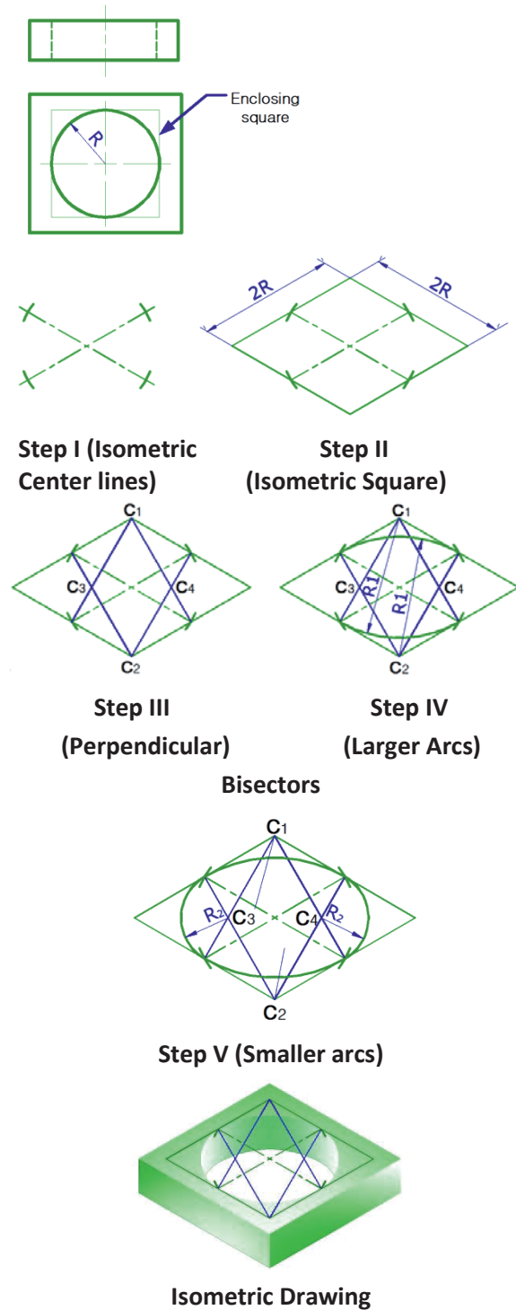
Fig. 7.18 Construction of isometric circle using four center method
