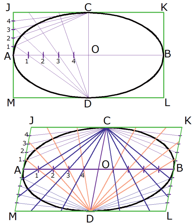
Fig. 5.47 Constructing an ellipse by parallelogram method
