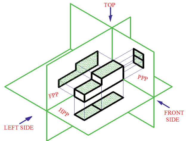
Fig. 6.5 First angle projection
