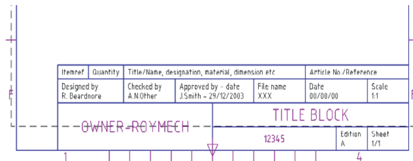
Fig. 2.32 Typical example of title block
