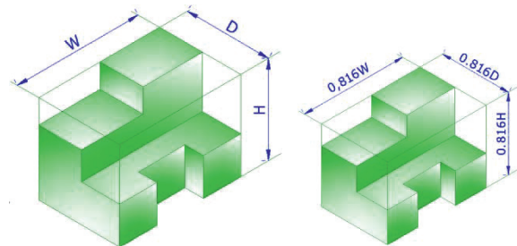
a) Isometric drawing b) Isometric projection
