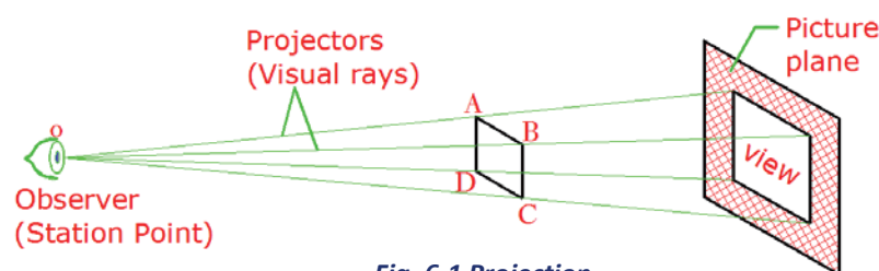
Fig. 6.1 Projection
