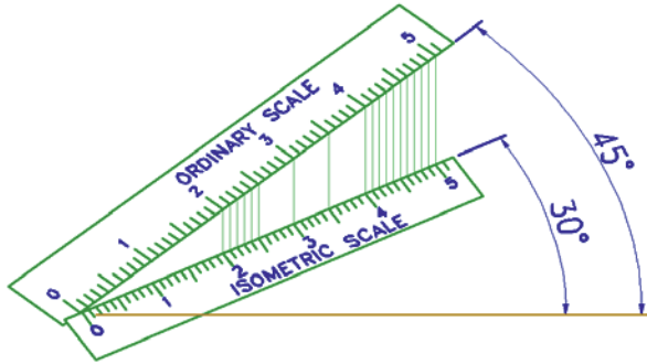
Fig. 7.9 Isometric scale
