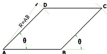
Fig. 5.26 Constructing a rhombus given side and included angle
