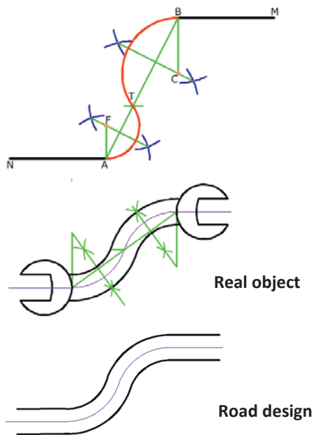
Fig. 5.43 Drawing ogee curve that connect lines
