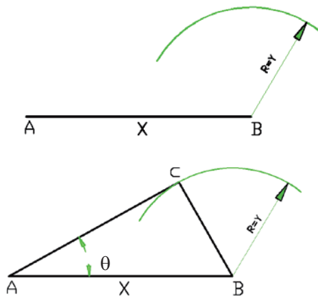
Fig. 5.13 Sine method
